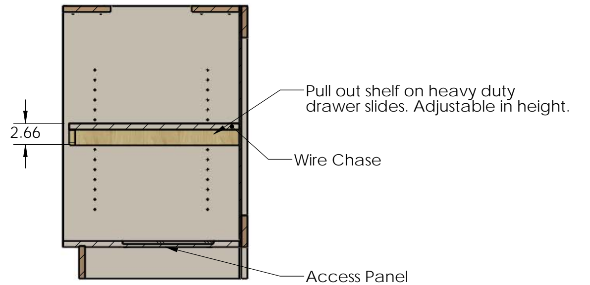
SECTION B-B
