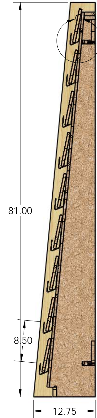
SECTION B-B
