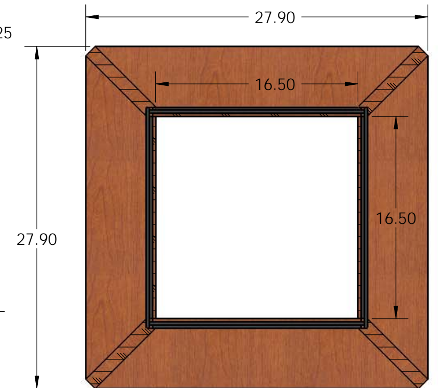
SECTION B-B
